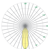
NRW 34° Beam
