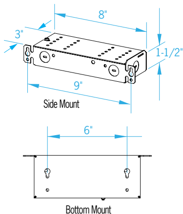
8" Box Dimensions
