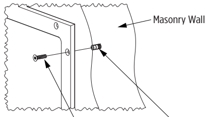
MMH – Masonry Mounting Hardware for masonry, cement or brick
