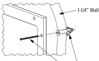
LMH – Long Mounting Hardware for 1-1/2" wall, double thickness 5/8" wallboard and/or wood
