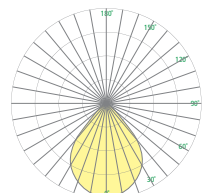
WIDE 84° Beam
