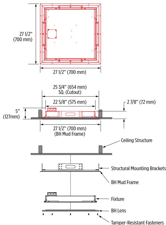
Sheetrock Installation BHSRI & BHSRI(IP65) Detail
