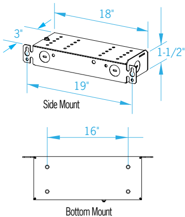
18" Box Dimensions
